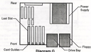
Diagram G Amiga 200 Top View
