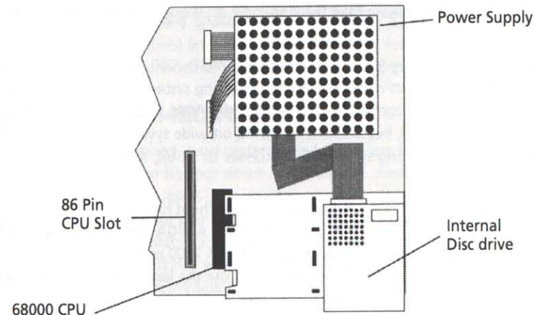
Illustration 4. Right side view (looking down)
