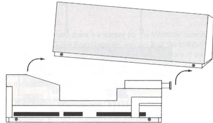
Illustration 3. Cover removal – side view
