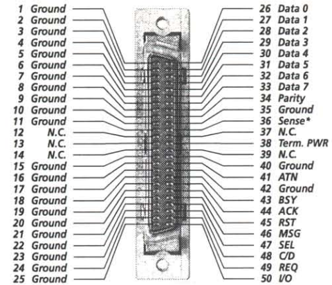
External SCSI-socket at the BLIZZARD 2060 Turbo Board (SCSI-II 50-pole)
