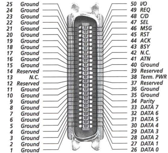
Connection cable assignment (Centronics 50-pole)
