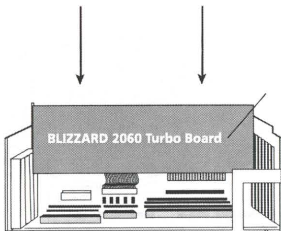
Illustration 5. BLIZZARD 2060 installation (side view)
