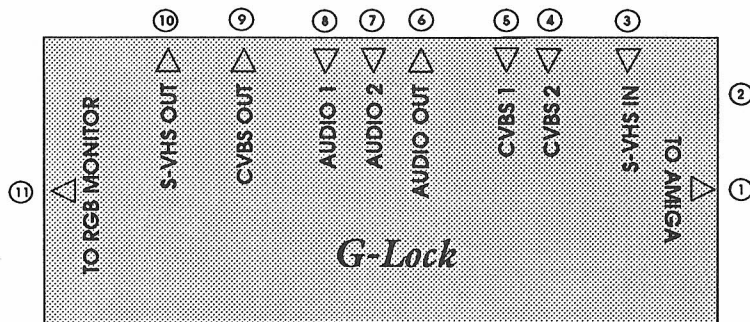
Figure 4.1 – G-Lock Connections
